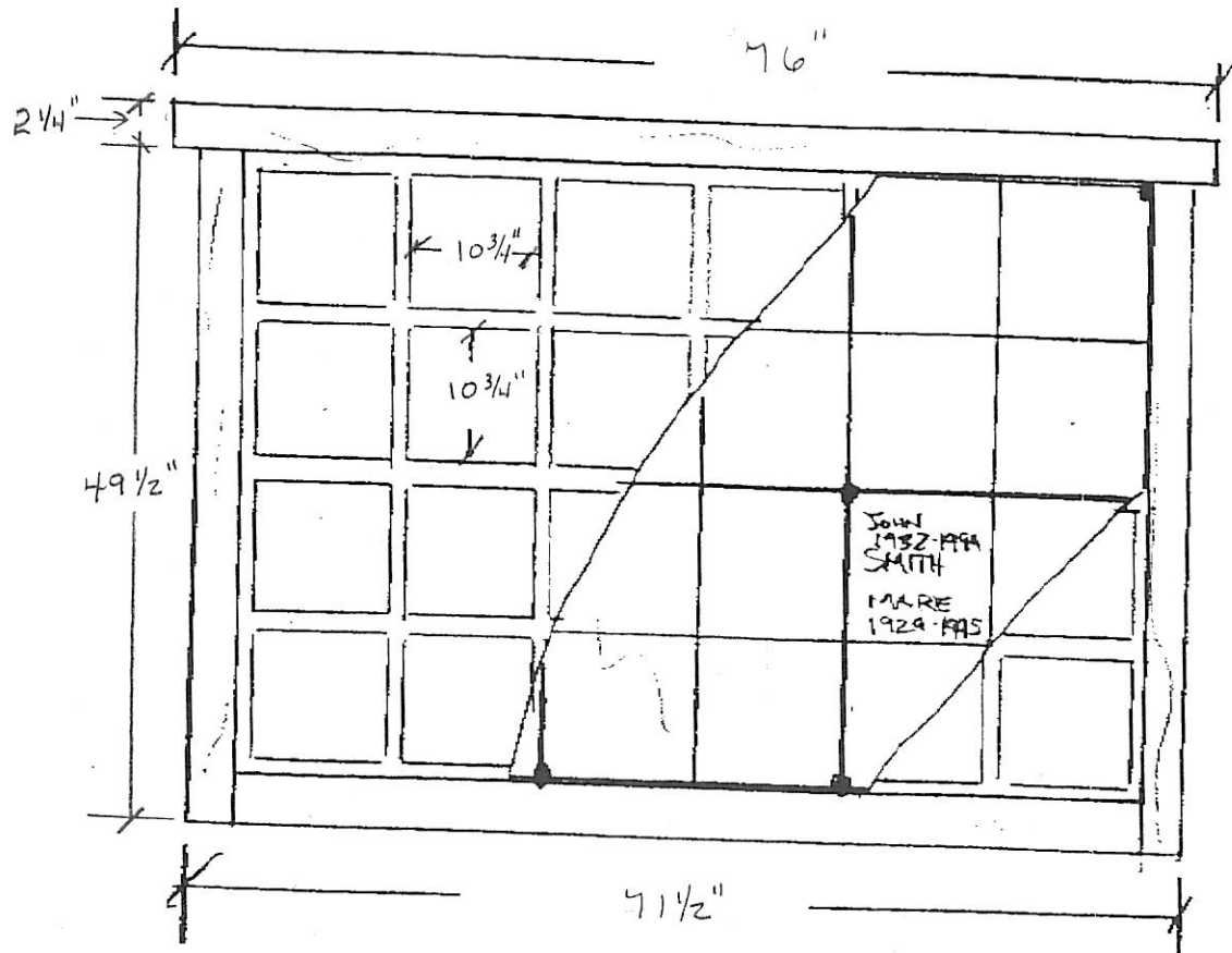
FACE ELEVATION (TYPICAL BOTH SIDES)
