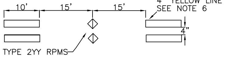
REVERSIBLE LANE LINE
