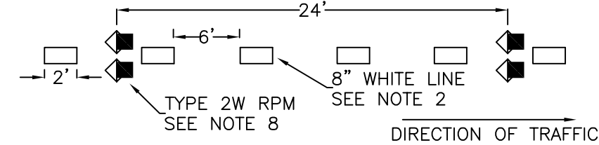
DOTTED WIDE LINE (DWL)
