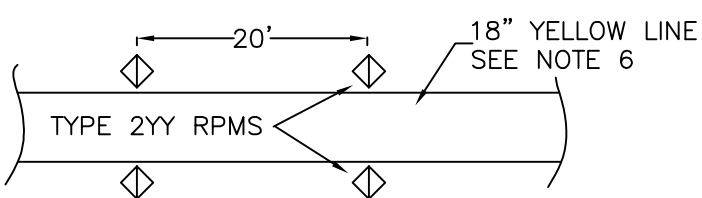
BARRIER LINE (BL)
