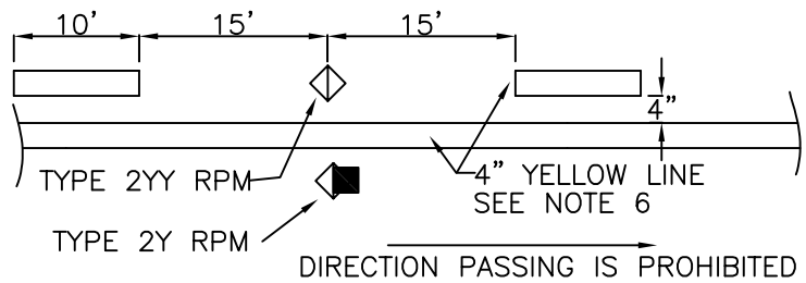
NO PASS LINE (NPL)
