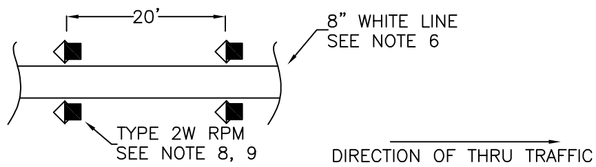
WIDE LINE (WL)
