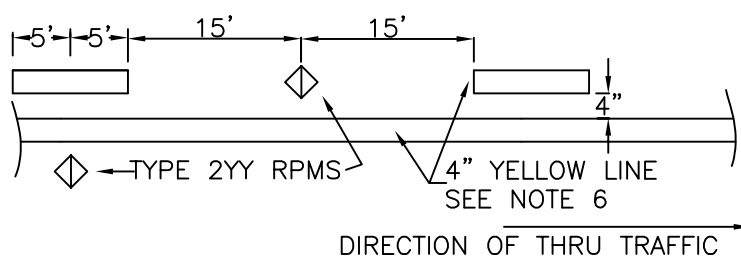
TWO-WAY LEFT TURN LINE (TWLTL)
