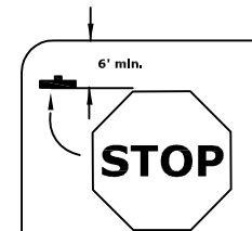
Typical Placement Plan
