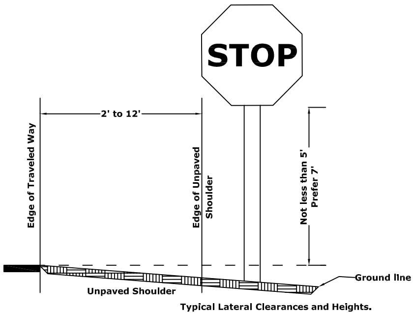
Typical Lateral Clearances and Heights.
