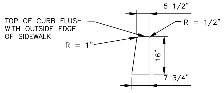
DETAIL A - CONCRETE BARRIER CURB
