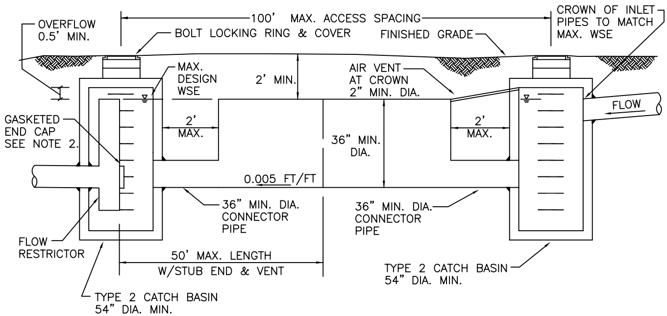
ELEVATION VIEW
