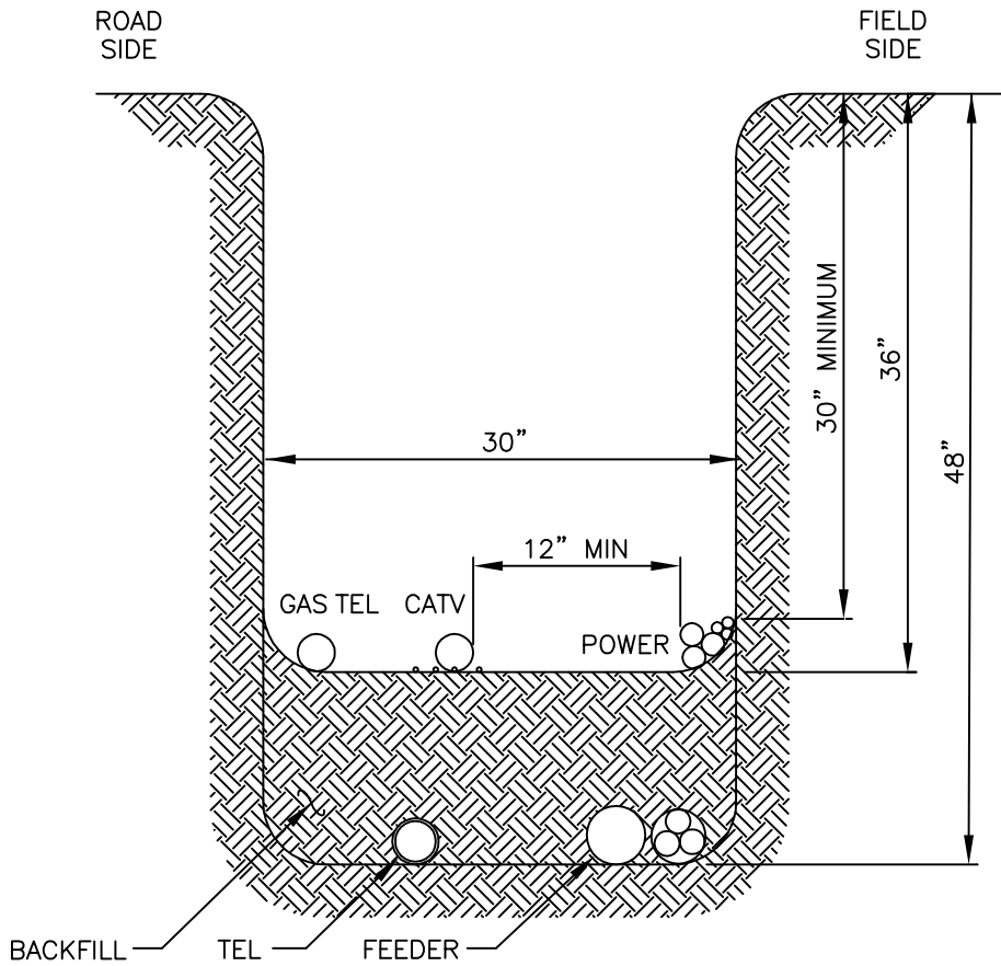
TYPICAL JOINT TRENCH CROSS SECTION
