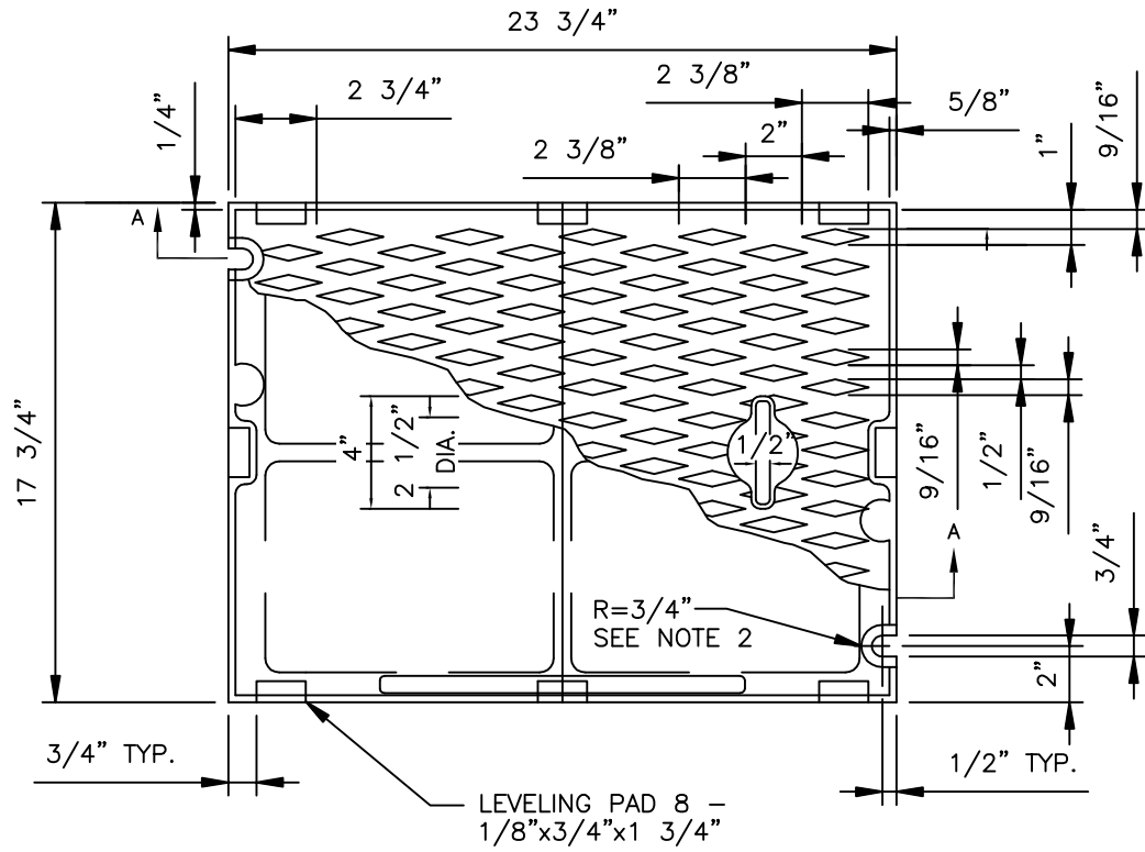
PLAN COVER
