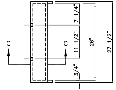
HOOD DETAIL
