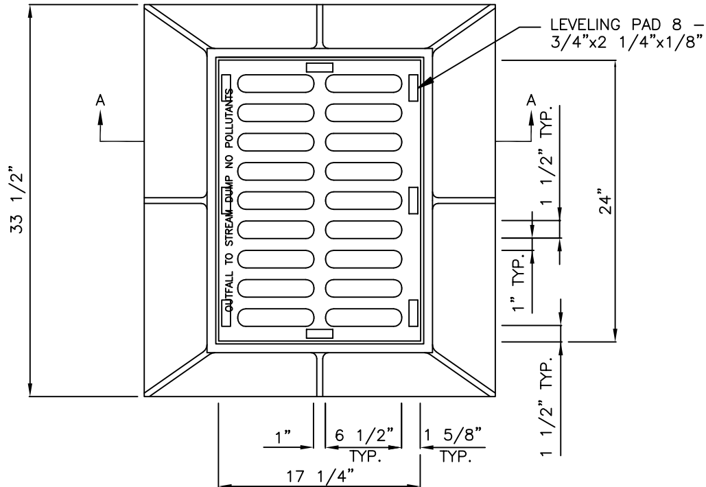
PLAN
