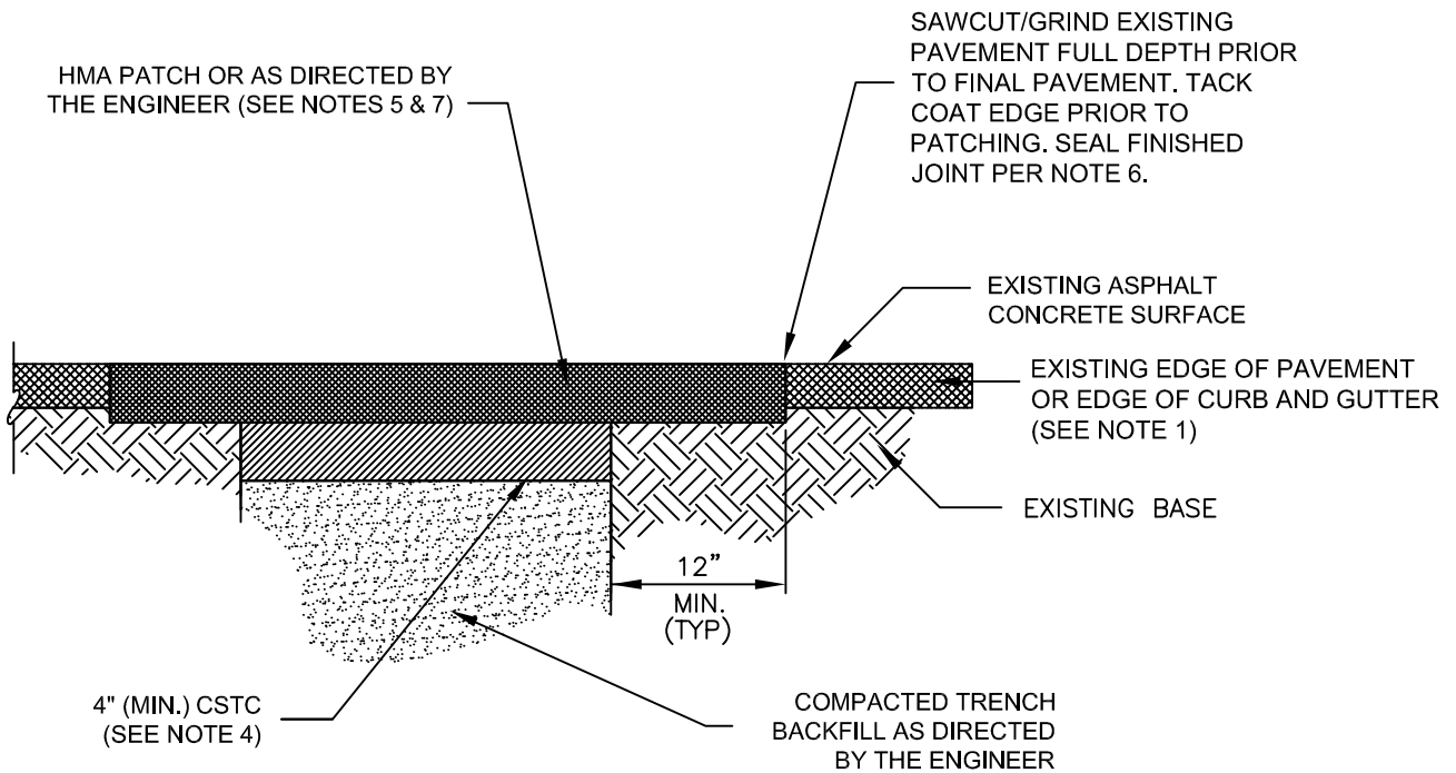
TYPICAL PATCH FOR PAVEMENT NOT TO SCALE
