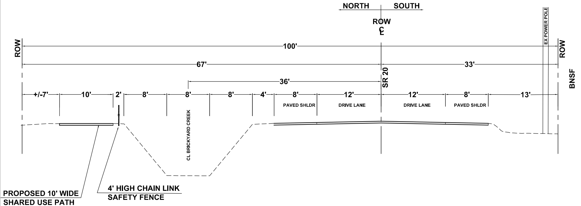
TYPICAL SHARED USE PATH SECTION STA 30+90 TO STA 53+05 SR20 MP 63.64 TO 64.06
